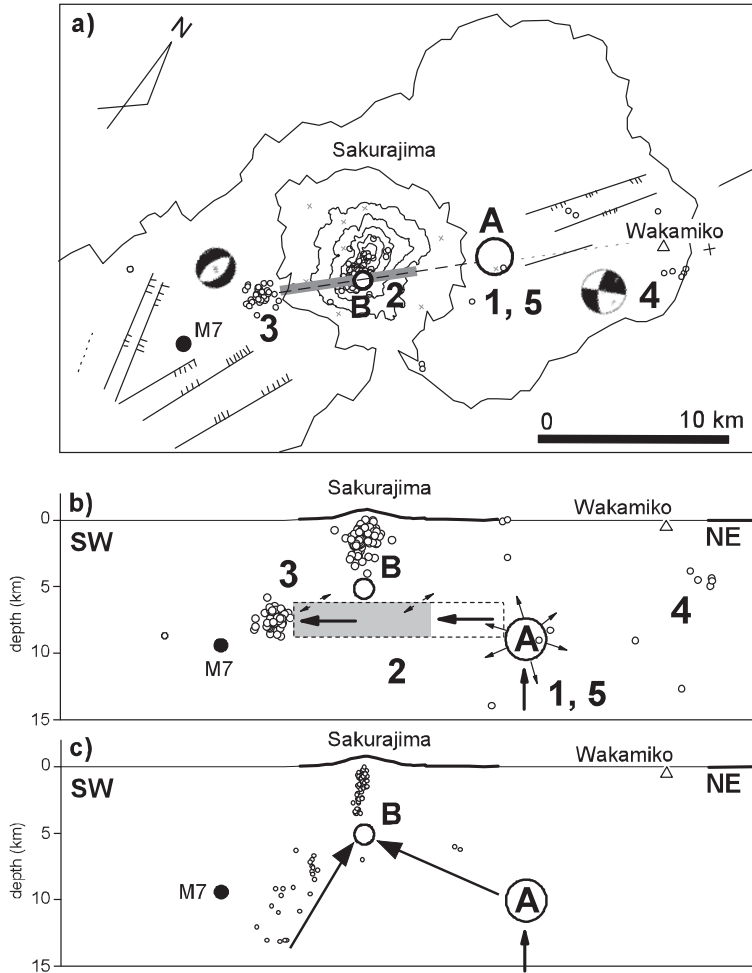
Fig. 10. Models of magma migration toward the Sakurajima volcano. A hypothetical model of the magma supply system at the Sakurajima volcano. (a) Horizontal plane and (b) vertical cross-section in the SW-NE direction (Hidayati et al. , 2007). The numbers correspond to volcanic processes during the period from 1999 to 2005. The open circles indicate VT earthquakes. The open circles with “A” and “B” are pressure sources beneath the Aira caldera and Sakurajima, respectively. The tensile fault is indicated by the rectangular dashed line, and the active zone from 2000 to the middle of 2004 is shown in gray. The inferred magma migration is indicated by arrows. The solid circle with M7 indicates the location of the largest earthquakes for the 1914 eruption as determined by Abe (1981). The lines with branches indicate geological faults, most of which are normal faults. (c) Previous model modified from Kamo (1988). The VT earthquakes that occurred during the period from 1976 to 1980 are plotted.
