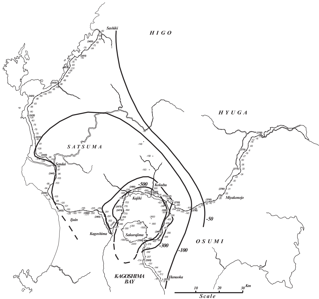
Fig. 3. Spatial distribution of height difference in south Kyushu before and after the 1914 eruption of Sakurajima (modified from Omori, 1916). Benchmarks are indicated by dots with numbers in brackets, and contours lines indicate isobaths in millimeters.
