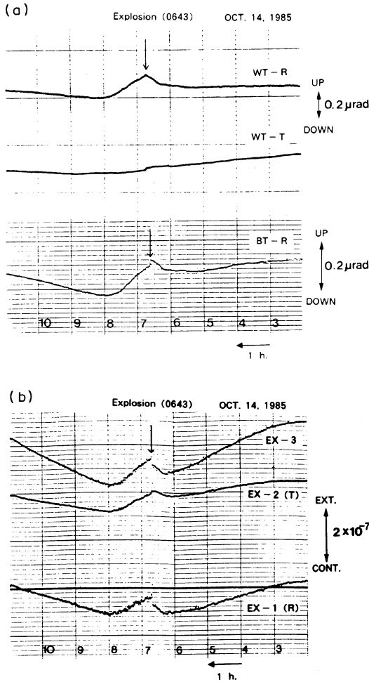
Fig. 15. (a) Tilt and (b) strain changes associated with vulcanian eruption (Ishihara, 1990). (a) “WT-R” and “WT-T” indicate the radial component from the crater and component tangential to the crater, respectively, as recorded by the water-tube tiltmeter in an underground tunnel at Harutayama (Fig. 1). “BT-R” is the radial component of the borehole tiltmeter at a depth of 290 m beneath Harutayama. (b) Extensometer records. EX-1: radial, EX-2: tangential, and EX-3: oblique components in the underground tunnel. The upward tilt of the crater side and the extension strain change started at 8 h.
