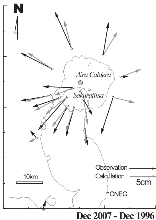
Fig. 6. Horizontal displacement vectors during the period from December 1996 to December 2007 (Iguchi et al. , 2008a). The solid and gray arrows show the observation and calculated vectors, respectively. The gray circle indicates the location of the Mogi pressure source. Station ONEG is used for reference.
