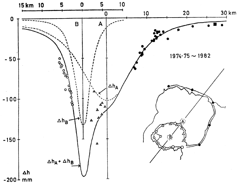
Fig. 7. Vertical displacement fitted by the theoretical value of sources A and B (Eto and Nakamura, 1986). The depths of sources A and B are 10 km and 3 km, respectively. The dashed curves \Delta h_A and \Delta h_B indicate the displacements induced by individual sources A and B, respectively, and the solid curves are the sums of \Delta h_A and \Delta h_B on the line passing through sources A and B. The dots, triangles, and open circles indicate the vertical displacements at the east and north rims of the Aira caldera, at the south and west parts of Sakurajima, and at the east and north parts of Sakurajima, respectively. The locations of the benchmarks are shown on the map, although some are omitted.
