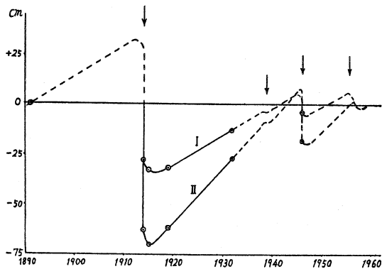
Fig. 4. Secular change in vertical displacement after the 1914 eruption (Sassa, 1956) I: BM2480, II: BM2474. See the locations of the benchmarks in Figs. 1 and 3. The dashed curves indicate estimations, and eruptions are indicated by arrows.
