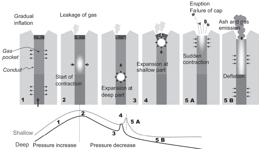
Fig. 16. Process of explosive eruption based on observations at Sakurajima, Semeru, and Suwanosejima volcanoes (Iguchi et al. , 2008b). Inferred pressure changes are shown at the bottom. “Shallow” and “Deep” indicate pressure changes at the upper part (less than 0.5 km) and the deep part (approximately 2 km) of the conduit. The difference is recognized at the Sakurajima volcano, and only changes at the shallow parts are detected at Suwanosejima and Semeru volcanoes. (1) Ascent of magma and the accumulation of volcanic gas in the conduit below a confining cap (plug). Pressure and volume increases are observed as inflation-related tilt/strain and upward displacement. (2) Release of gas as the gas pressure exceeds the strength of the cap. The resultant minor contraction is detected as deflation tilt and downward displacement. (3) Pressure decrease in the conduit starting from the gas pocket, inducing sudden outgassing of water-saturated magma deep in the conduit. Expansion is detected by upward P-wave first motion of the explosion earthquake. (4) Expansion process destroying the cap at the top of the conduit. Stages (3) and (4) could not be distinguished at the Suwanosejima and Semeru volcanoes. (5A) Failure of the cap at the top of the conduit. The gas pocket at the upper part of the conduit collapses, inducing a contraction ground deformation source at the shallow part. The deformation is revealed by the step of the crater-side-down tilt and the step of the tensional strain, as well as downward ground deformation. (5B) Ash and gas emission from the conduit. Pressure and volume decreases are observed as deflation-related tilt/strain and downward displacement, respectively.
