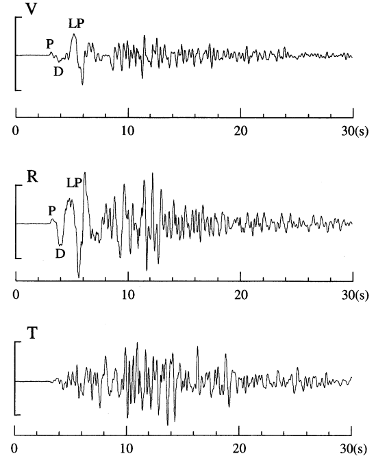
Fig. 17. An example of velocity seismograms of an explosion earthquake (Tameguri et al. , 2002). The explosion occurred at 04h55 m, September 3, 1999. “V” is the vertical component of the broadband seismometer, and “R” and “T” represent the horizontal components radial from the crater and tangential to the crater, respectively. “P”, “D”, and “LP” indicate the characteristic phases of the explosion earthquake. “P” refers to the P-wave first motion with compression onset. “D” refers to the subsequent dilatational P-wave. “LP” refers to the long-period Rayleigh wave.
