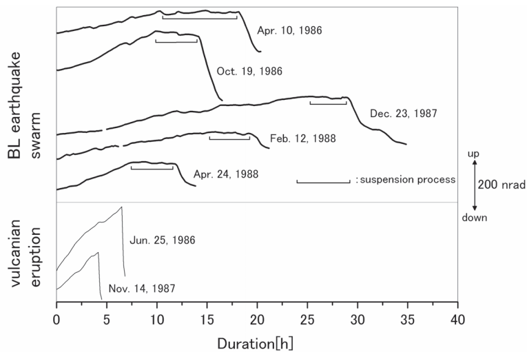
Fig. 13. Examples of tilt change associated with a BL-type earthquake swarm (upper) and vulcanian eruption (lower). Eruptive activity continued during the downward tilt of the crater side (Tateo and Iguchi, 2009). Tilts were observed at the underground tunnel at Harutayama (Fig. 1). The upward tilt of the crater side changes to downward tilt after a short period of deadlock, as indicated by the suspension process.
