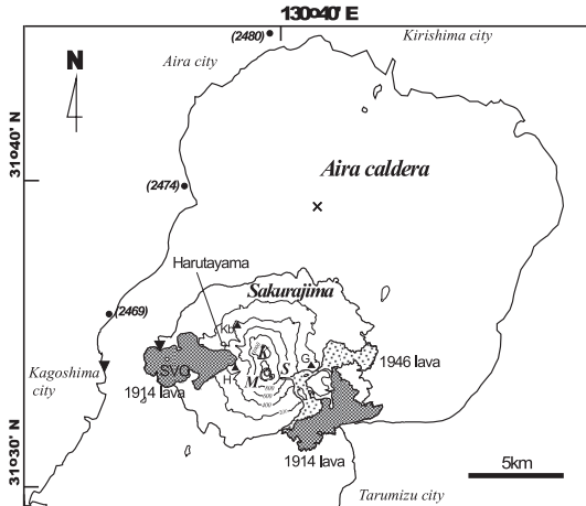
Fig. 1. Map of Sakurajima and the Aira caldera. The dots indicate important benchmarks referred to in the text, and the inverted triangles indicate tide gauges. The central cones and craters are K : Kitadake, M : Minamidake, and S : Showa crater. Representative parasitic cones are indicated by triangles ( H : Hikinohira, G : Gongen-yama, and Kb : Kabano). Cross represents a pressure source location obtained by Mogi (1958).
