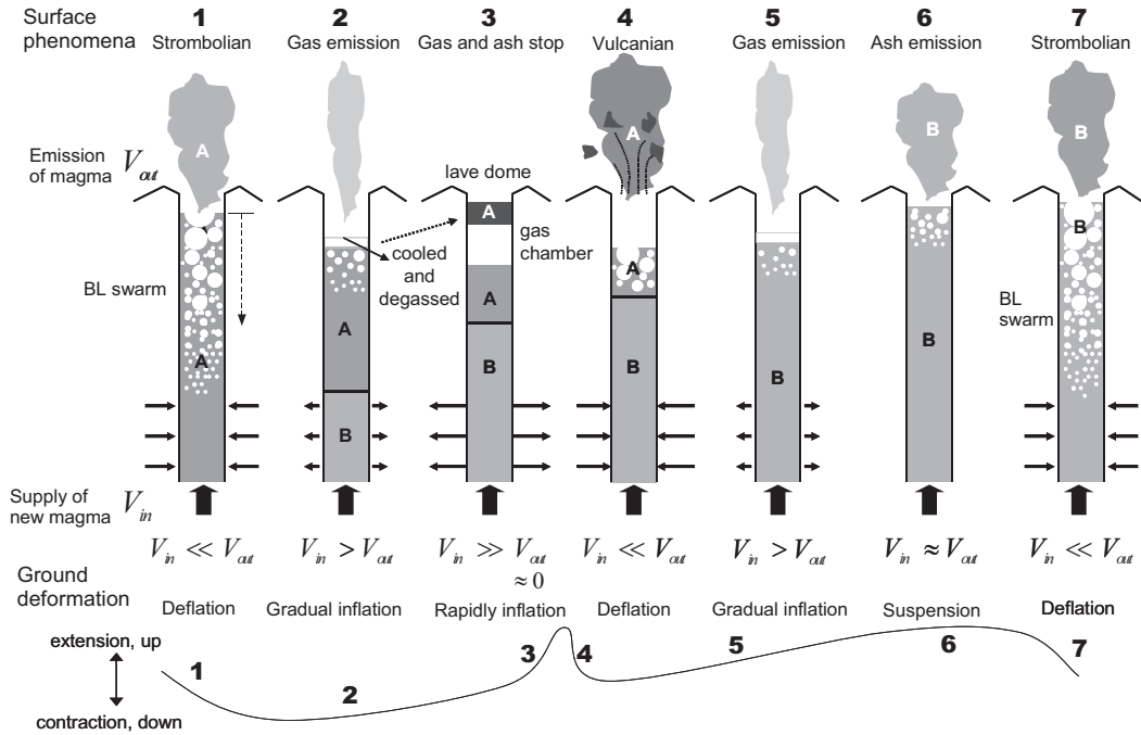
Fig. 14. Schematic diagram of the internal change of the conduit inferred from ground deformation and surface phenomena (Tateo and Iguchi, 2009). V_{in} indicates the volume of magma supplied from the magma reservoir, and V_{out} indicates the volume of magma emitted as volcanic ash and gas. The symbols “A” and “B” represent magma that was supplied to the conduit in different stages. The inward and outward arrows indicate deflation and inflation of the deep part of the conduit, respectively. Larger volume changes are indicated by larger arrows. A schematic diagram of the ground deformation of tilt and strain changes is shown at the bottom of the figure.
