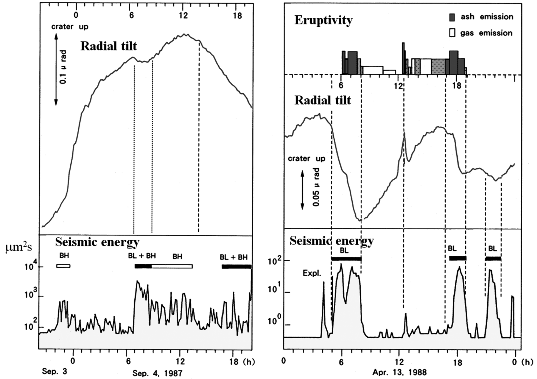
Fig. 12. Tilt changes associated with swarms of BL-type earthquakes (a) and BH-type earthquakes (b) (modified from Ishihara and Iguchi, 1989). Tilts were observed at the underground tunnel at Harutayama (Fig. 1). (a) The seismic energy at station HIK (Fig. 1), which is 1.7 km from the summit crater, is shown in the lower part of the figure, and the temporal change of the eruptive activity associated with the BL-type earthquake swarm is shown in the upper part of the figure. No significant changes in surface phenomena were detected in the BH-type earthquake swarm.
