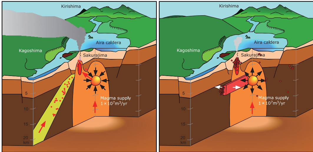
Fig. 18. Image of magma supply beneath the Sakurajima volcano. (a) 1974–1992 (modified from Kamo, 1988) when vulcanian eruptions reoccurred at the Minamidake crater. (b) after 1993 (modified from Hidayati et al. , 2007) when the eruptive activity decreased.
