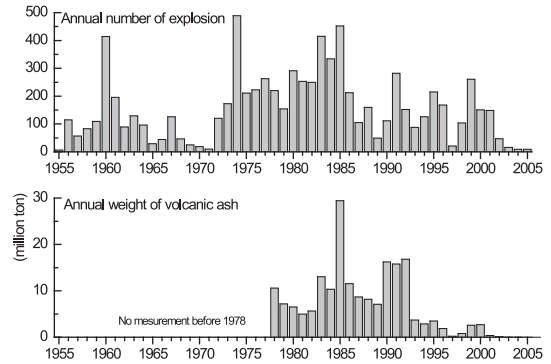
Fig. 2. Annual numbers of vulcanian eruptions and weights of volcanic ash ejected from the Minamidake crater during the period from 1955 to 2005. Observation of weight of volcanic ash started in 1978 by the Kagoshima Prefectural Government.
