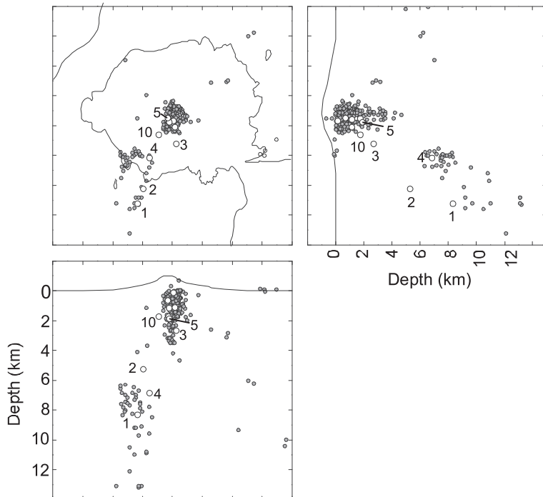
Fig. 8. Hypocenter distribution of A-type earthquakes during the period from 1976 to 2004. The numbered white circles represent the hypocenter location as determined by Kamo (1978) and indicate the order of earthquake occurrence prior to the increase in eruptive activity in May 1976. The numbers 6 through 9 are omitted in order to avoid congestion. These hypocenters are located at depths of less than those of events 5 and 10 beneath the Minamidake.
