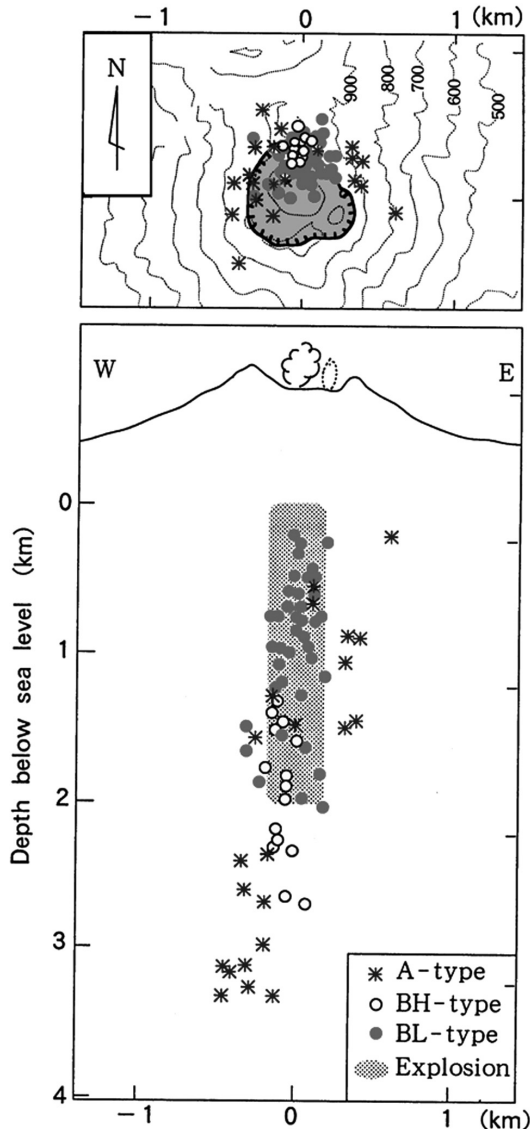
Fig. 11. Hypocenter distribution of A-type, BH-type, and BL-type earthquakes and explosion earthquakes during the period from 1987 to 1988 (Iguchi, 1994). Top: epicenter distribution. Bottom: hypocenter distribution on the cross-section in the east-west direction. The shaded area indicates the hypocentral zone of the explosion earthquakes (Ishihara, 1990)
