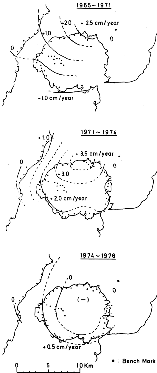
Fig. 9. Distribution of vertical displacement in three periods (Ishihara and Eto, 1978). The displacement is in reference to BM.2469 (Fig. 1), and the elevation at Sakurajima is connected by the tide difference between two ports: Kagoshima and Hakamagashi in Sakurajima (see Fig. 1). Top: the vertical displacements at the northern part are maximal. Middle: the entirety of Sakurajima is uplifted higher than Kagoshima. Bottom: the number of explosive eruptions increased. Ground deformation revealed no uplift or subsidence, particularly at the NE part.
