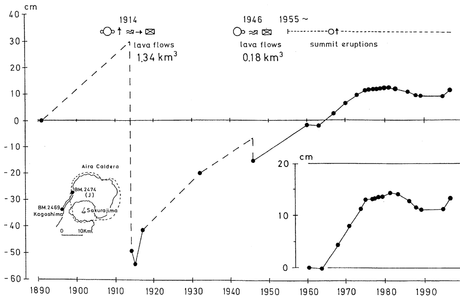
Fig. 5. Secular changes in the relative heights of BM.2474 referring to BM.2469 and the volcanic activity at Sakurajima (Eto et al. , 1997). The vertical displacement after 1960 is enlarged in a square in the lower-right corner. The dashed lines indicate an estimation based mainly on Sassa (1956). The volumes of the lava flows effused by the 1914 and 1946 eruptions are 1.34 \text{ km}^3 and 0.18 \text{ km}^3 , respectively.
